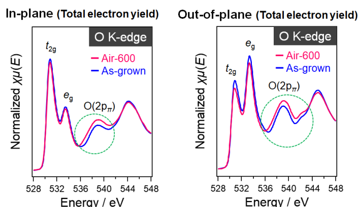
Fig. 1 O K-edge X-ray absorption spectroscopy (XAS) spectra for the as-deposited (blue), and annealed Nb-doped \text{TiO}_2 thin films at 600^\circ\text{C} (red). The internal angle between the incident X-rays and the z-axis on the substrate surface plane is set to \Psi = 0^\circ , and 70^\circ for in-plane and out-of-plane structural analysis, respectively.
