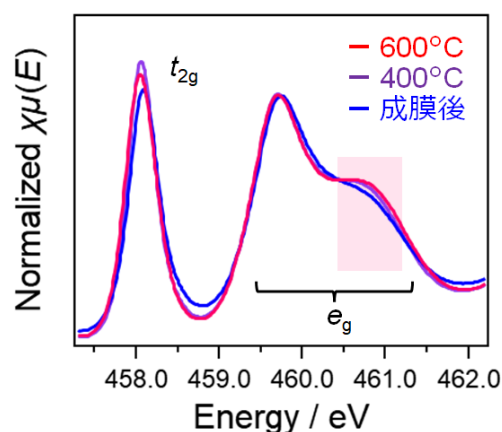
Fig. 1 Ti L III -edge X-ray absorption spectroscopy (XAS) spectra for the as-deposited (blue), and annealed Nb-doped TiO 2 thin films at 400 (purple) and 600°C (red). The internal angle between the incident X-rays and the z -axis on the substrate surface plane, \Psi = 0^\circ , with the polarization vector of the X-rays perpendicular nearly to the z and y -axes on the substrate surface, respectively.
