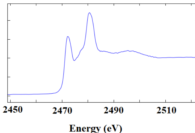
Fig. 1 S K-edge XAFS spectrum of the Fe-humate complex, prepared with amorphous Fe(III) oxides and Arako humic acids under pH 4, in relatively reduced state.
