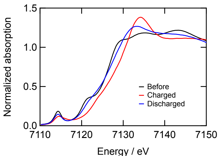
Fig. 1. Fe K-edge XANES spectra during charge and discharge.
