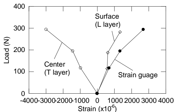
Fig. 1 Load-strain curve of OSB.
