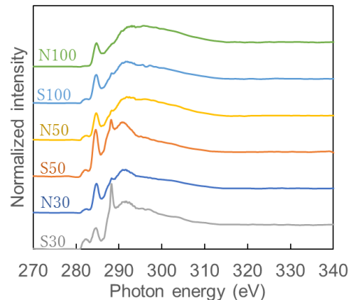
Figure 1. The NEXAFS C K-edge spectra of a-C films grown with different bias power and bias modulation. (S: With bias modulation, N: Without bias modulation, Num.: bias power)
